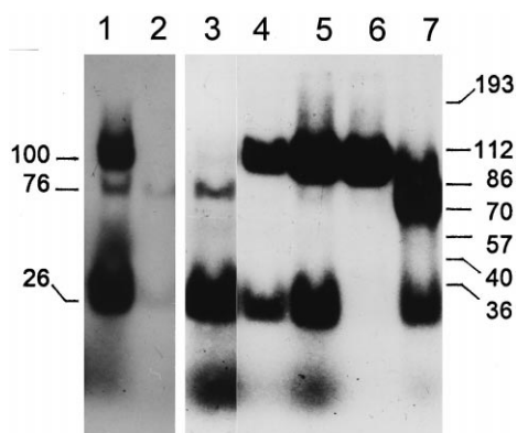
Fig. 1. Characteristics of phosphoprotein formation in the PM preparations from T. viridis . Phosphorylation for 30 s, hydroxylamine treatment and electrophoresis were carried out as described in Section 2. Lane 1, the standard reaction mixture, buffer control to hydroxylamine treatment; lane 2, hydroxylamine treatment; lane 3, the standard reaction mixture lacking sodium; lane 4, the standard reaction mixture, sodium concentration enhanced up to 100 mM; lane 5, the standard reaction mixture lacking magnesium; lane 6, 30 s phosphorylation in the standard reaction mixture lacking magnesium followed by a 10 s chase with 5 mM unlabeled ATP; lane 7, the standard reaction mixture, magnesium concentration enhanced up to 5 mM.
